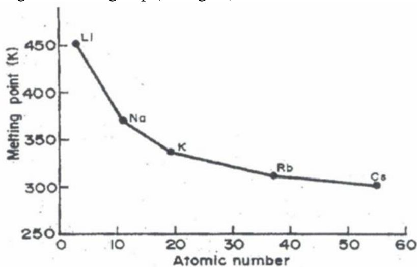
Fig 15: Trend in the melting point of Group 1 element Thermal and Electrical Conductivity
