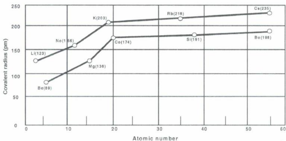
Fig 5. Plot of covalent radius against atomic number
