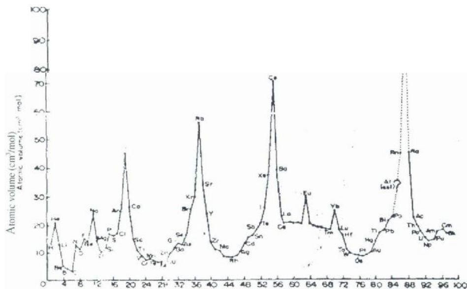
Figure 1. Periodic dependence of atomic volume on atomic number
