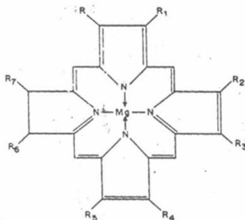
Fig 25: Skeleton of chlorophyll molecule
