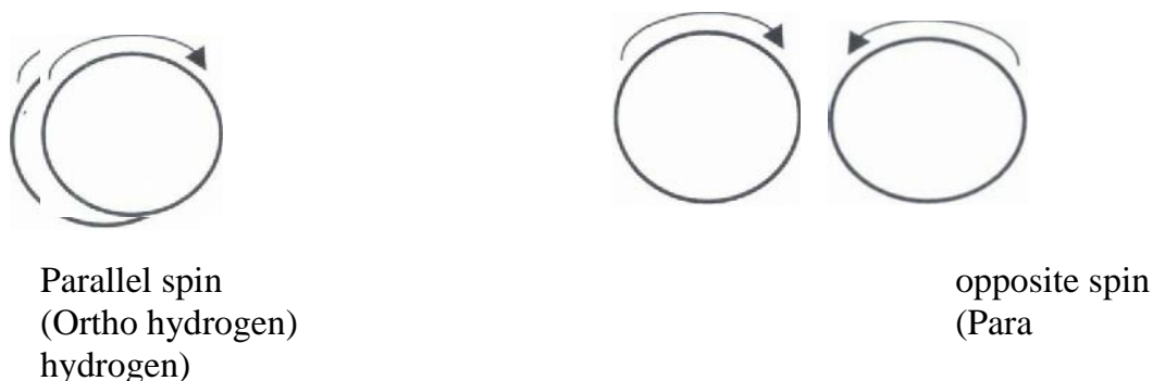
Fig .8: Ortho and Para forms of hydrogen
