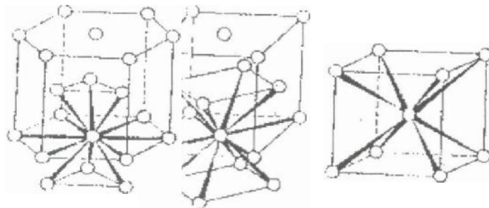
Fig. 4. Types of metallattices (a) hexagonal; (b) cubic close packed (c) body-centred cubic
