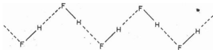
Hydrogen fluoride, (HF)_n
