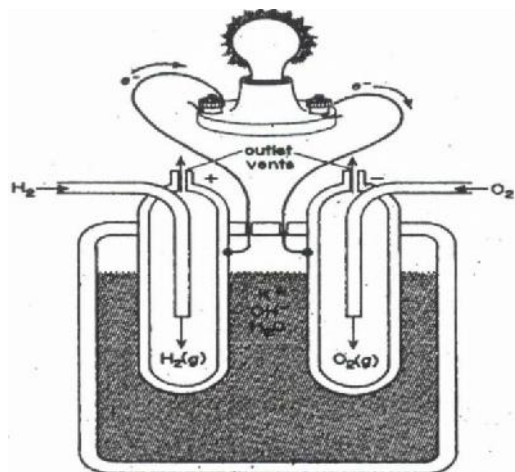
Fig 11: A hydrogen-oxygen fuel cell with KOH electrolyte and porous carbon electrodes
